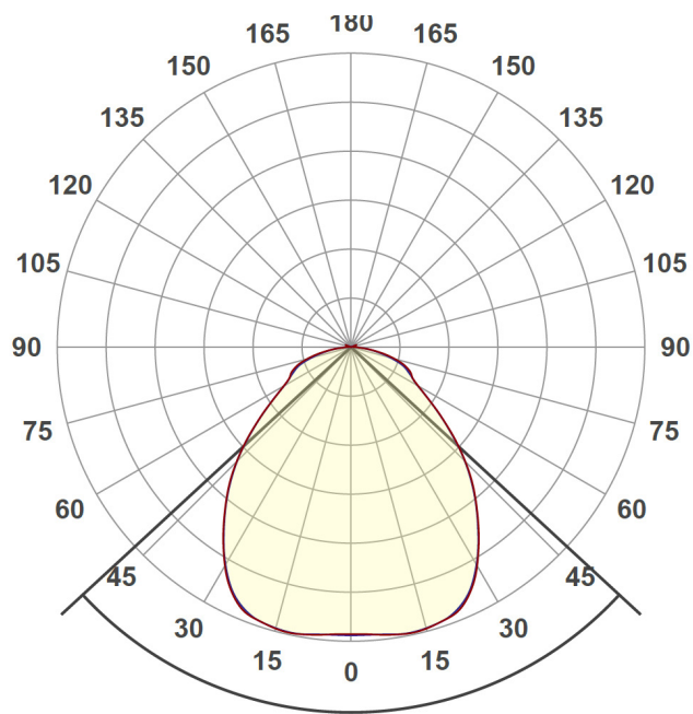
Beam angle: 94,6° Intensity distribution - Polar
