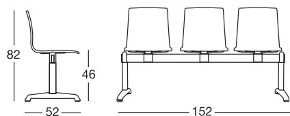
3 sedute 3-seater bench Art. 2761
