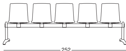
5 sedute 5-seater bench Art. 2763
